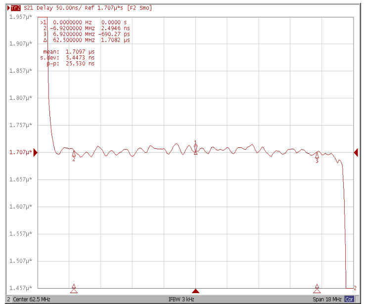
Group Delay Variation Fo±6.92MHz
