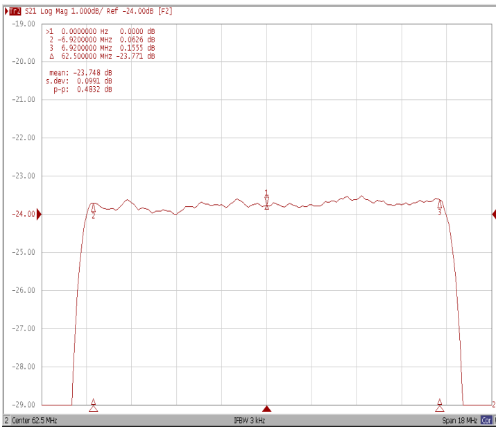
Ripple Variation Fo±6.92MHz
